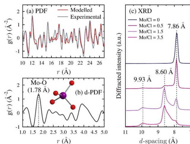
Fig. 3. (a): Experimental and modelled AFm-Cl PDF. (b): differential PDF (AFm-Cl minus a sample with Mo/Cl = 3.5). The Mo–O peak at 1.78 Å is diagnostic for \text{MoO}_4^{2-} (schematized in the inset). The peak at \sim 4 Å is due to Mo–Ca and Mo–Al correlations, consistent with \text{MoO}_4^{2-} in the interlayer mid-plane. (c): X-ray diffraction pattern of samples having Mo/Cl ranging 0–3.5. Peak asymmetry is due to interstratification (extracted from (Grangeon and Marty, 2019)).
